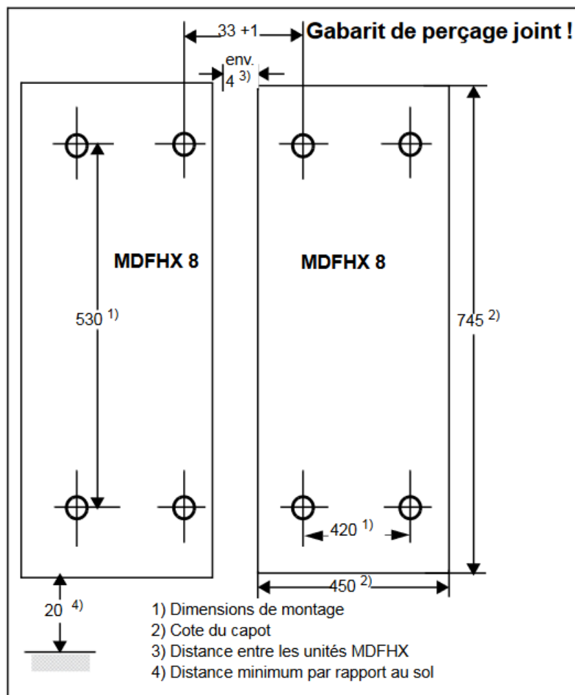
Figure 76: Montage de la fixation murale MDFHX 8
