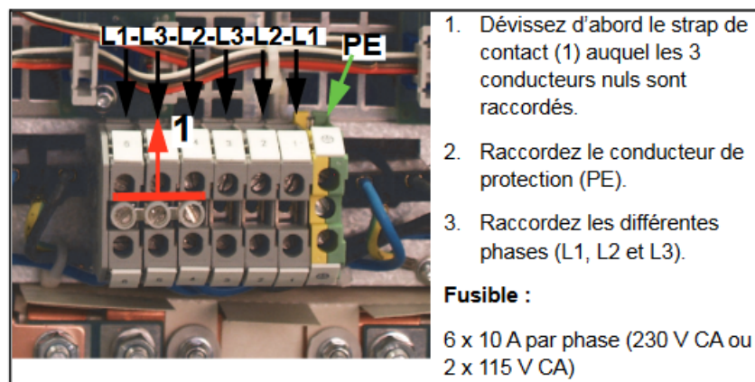
Figure 166: Raccordement circuit en triangle (PSR930/PSR930E)
