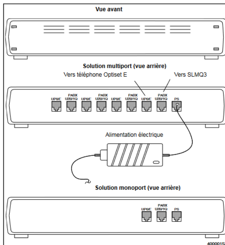
Figure 199: Adaptateur distant
