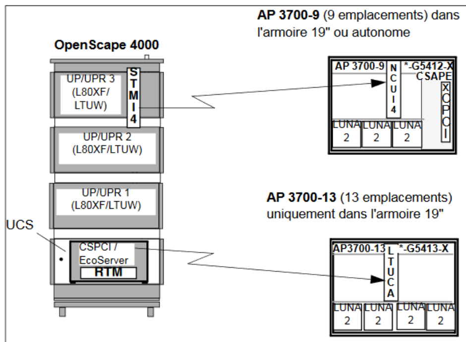
Figure 70: Raccordements AP 3700
