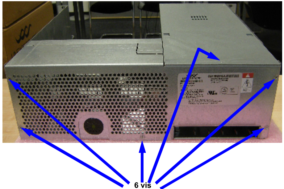
Figure 132: Capot arrière
