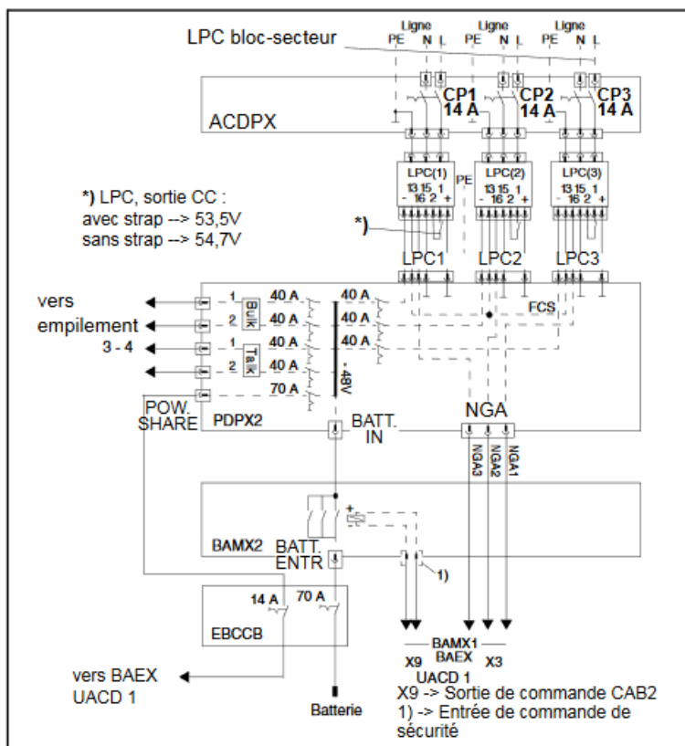
Figure 170: Raccordements UACD 2
