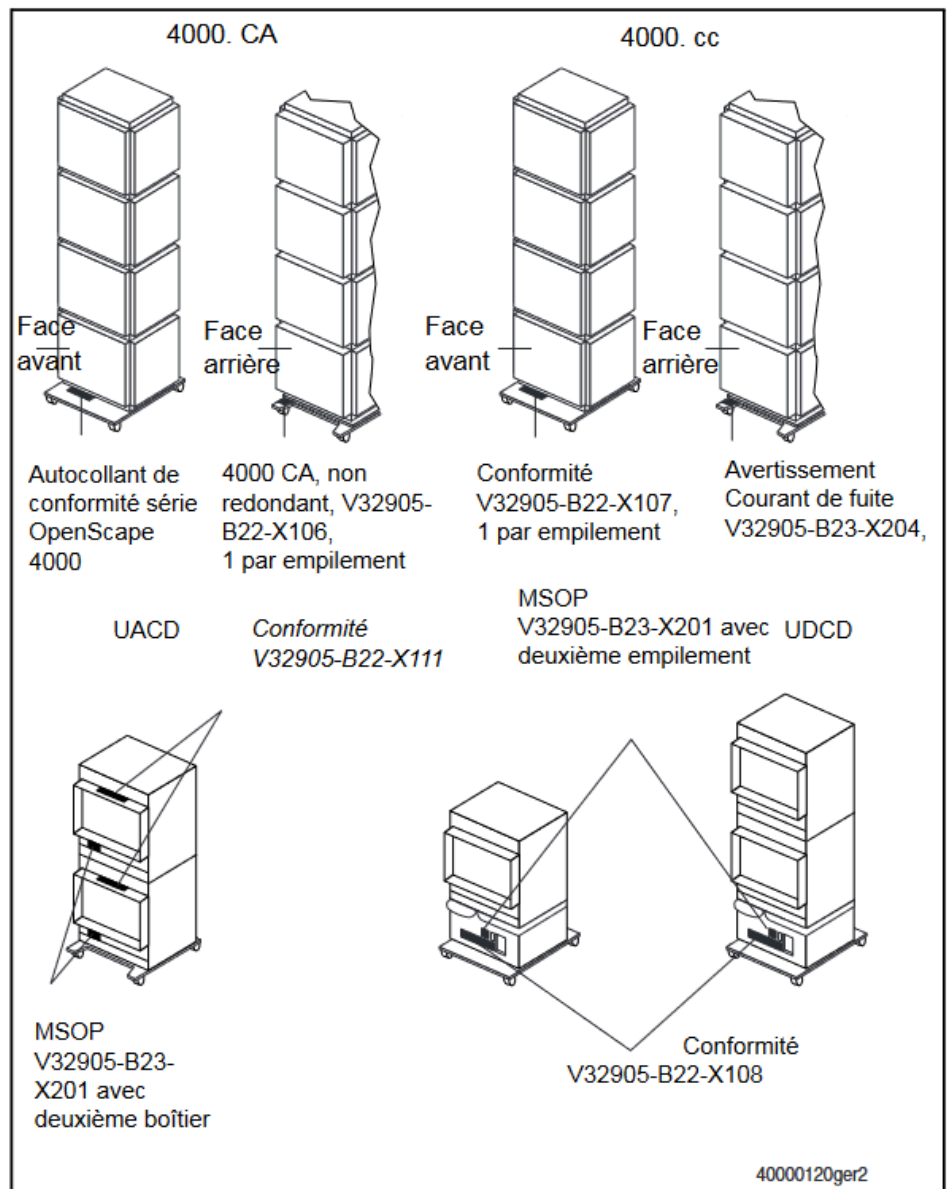
Figure 17: Position des autocollants
