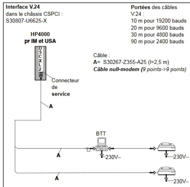
Figure 191: Raccordement du terminal
