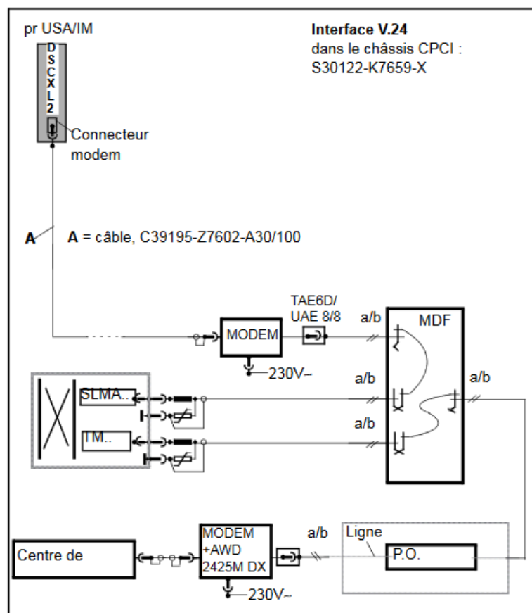
Figure 192: HiPath SIRA
