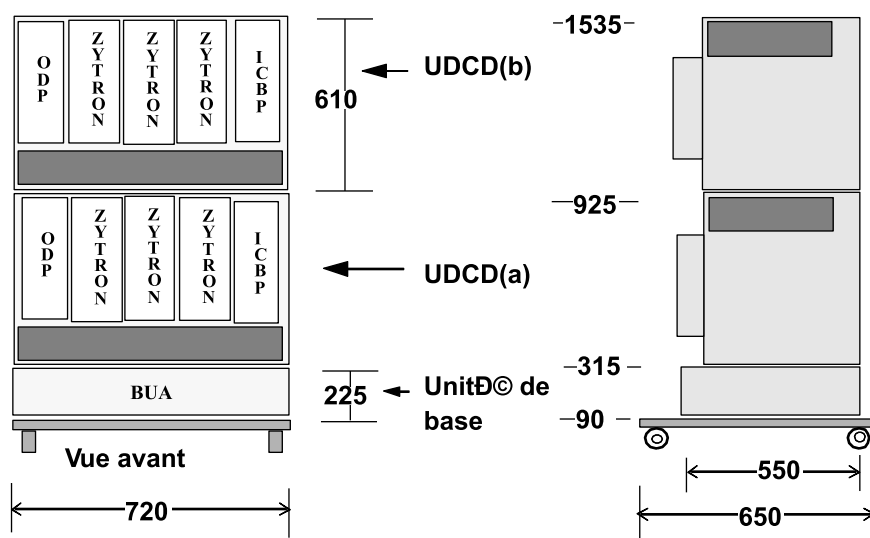
Figure 51: UDCD
