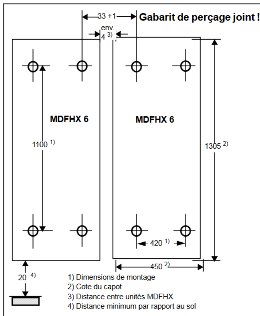
Figure 75: Montage de la fixation murale MDFHX 6
