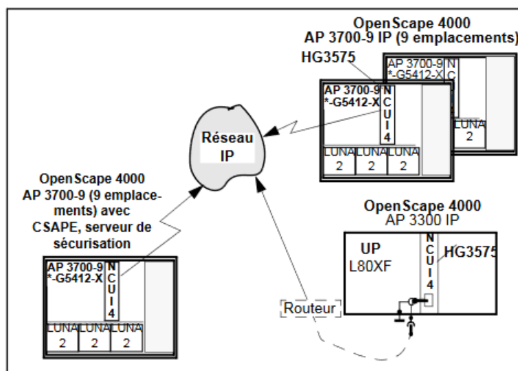
Figure 201: Raccordement IPDA sur AP 3700-9
