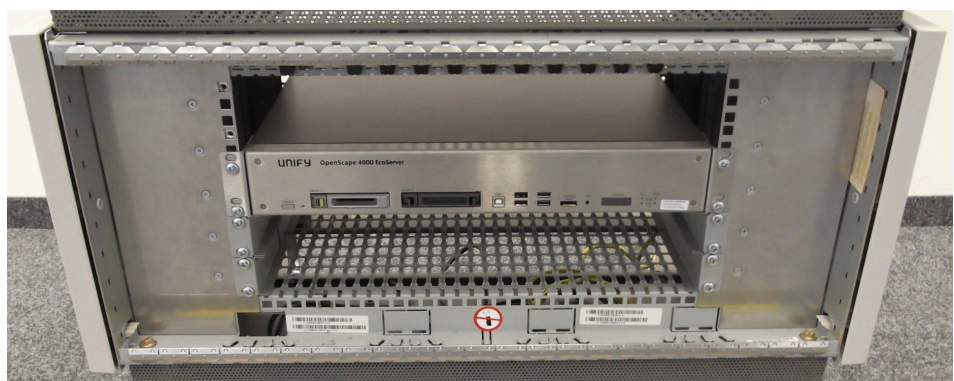
Figure 61: Structure 30"
