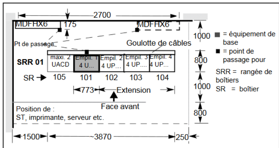
Figure 54: Montage au sol de OpenScape 4000 (variante 30")
