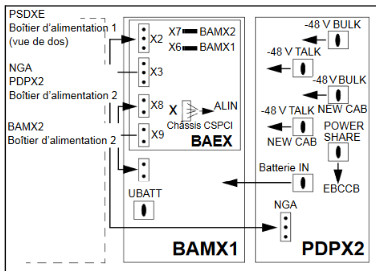
Figure 178: Raccordement PSDXE
