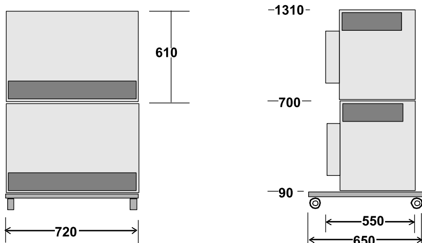
Figure 50: UACD
