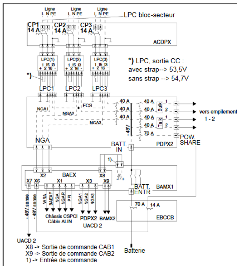
Figure 169: Raccordements UACD 1
