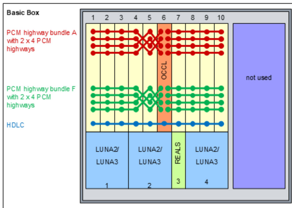
Abbildung 19: OpenScape Business X8 – PCM-Highways in der Basisbox
