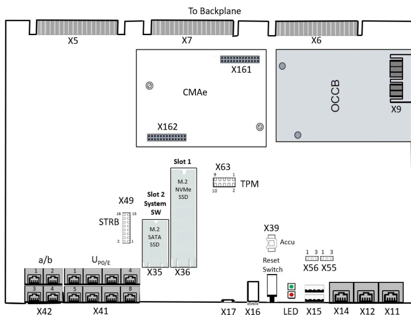
Abbildung 32: OCCMBR/OCCMAR - Anschlüsse
