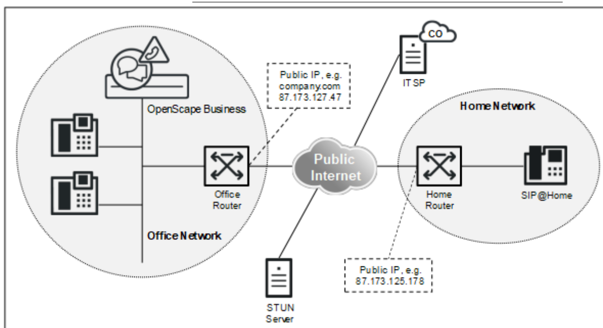
Figure 6: Device@Home (SIP Device@Home or System Device@Home) components
