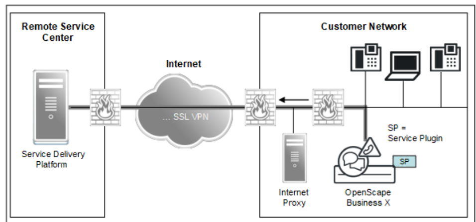
Figure 14: RSP - Overview for OpenScape Business X
