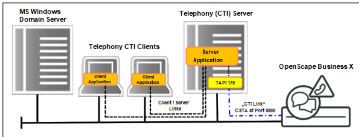
Figure 10: Server-Based TAPI Application via TAPI 170 to OpenScape Business
