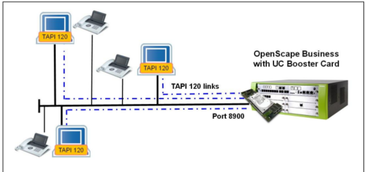
Figure 8: TAPI 120 in CSTA Mode with OpenScape Business X5R and UC Booster Card
