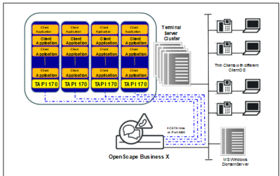
Figure 12: Client-Based TAPI Applications on Terminal Server to OpenScape Business
