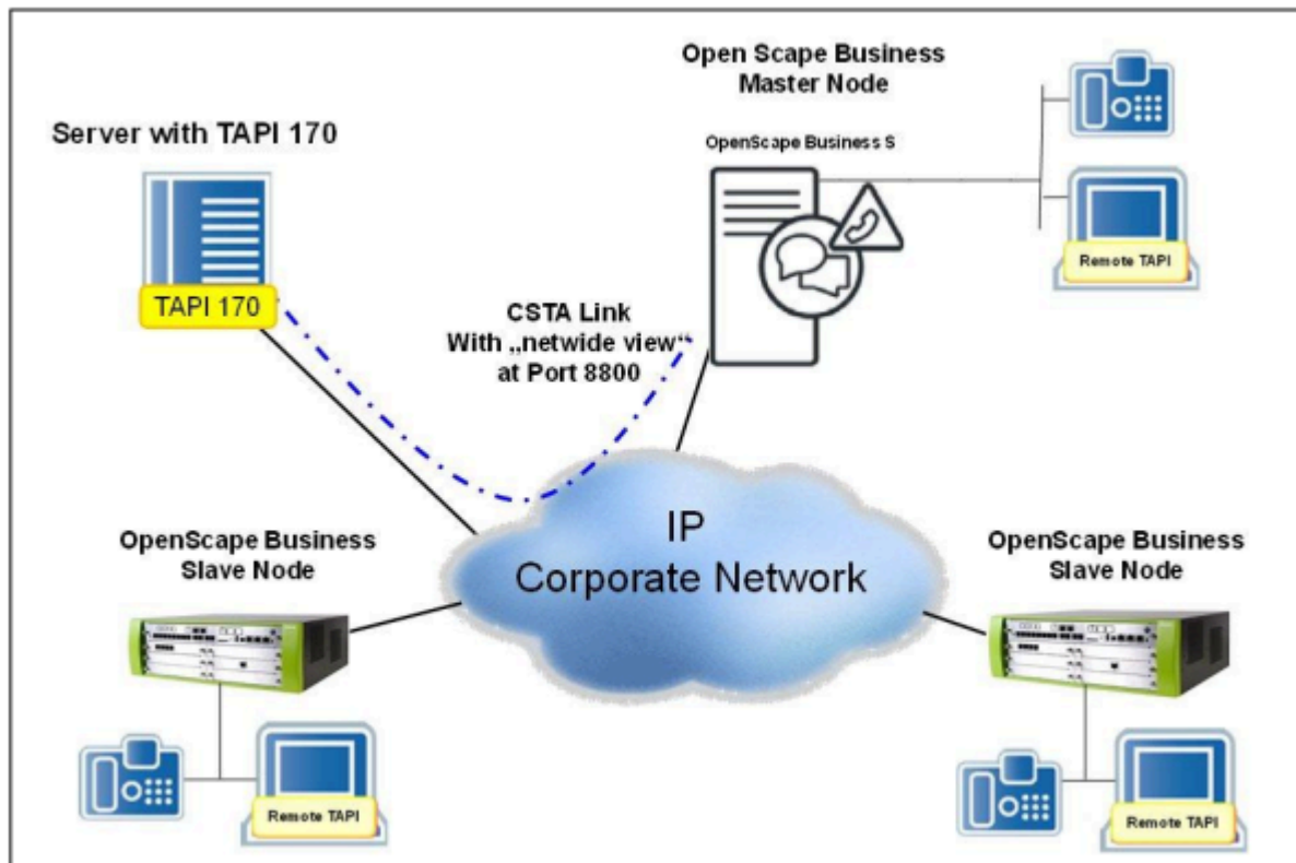
Figure 13: Connecting TAPI 170 to Networked OpenScape Business Systems
