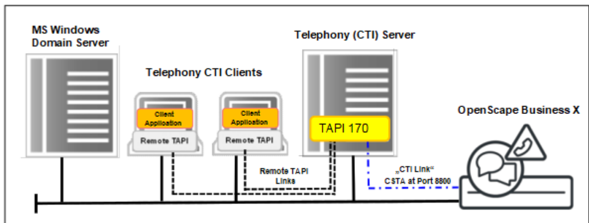
Figure 11: Client-Based TAPI Application via "Remote TAPI" to OpenScape Business
