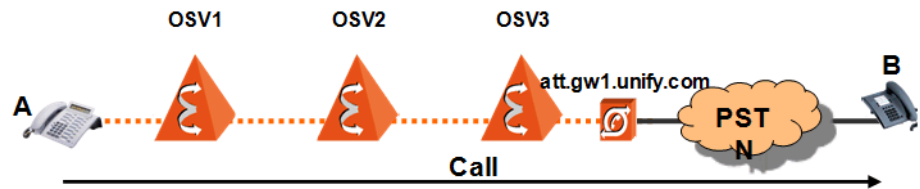
Figure 8 Outgoing Call Scenario
