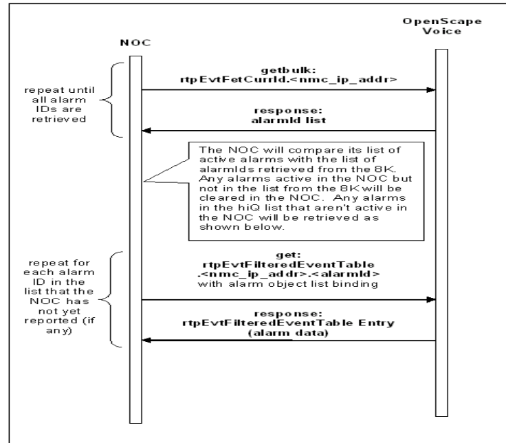
Figure 6 Filtered Alarm Audit and Resynchronization
