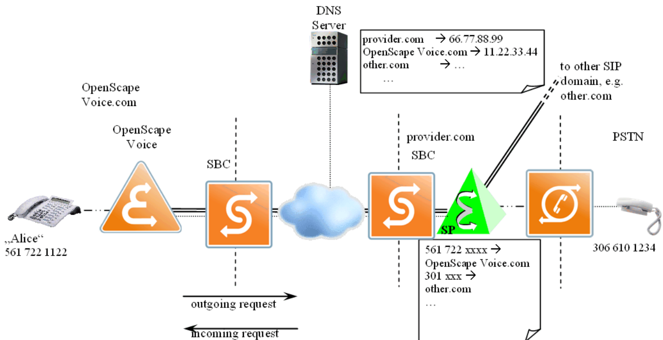
Figure 33 Example OpenScale Voice - Service Provider Configuration
