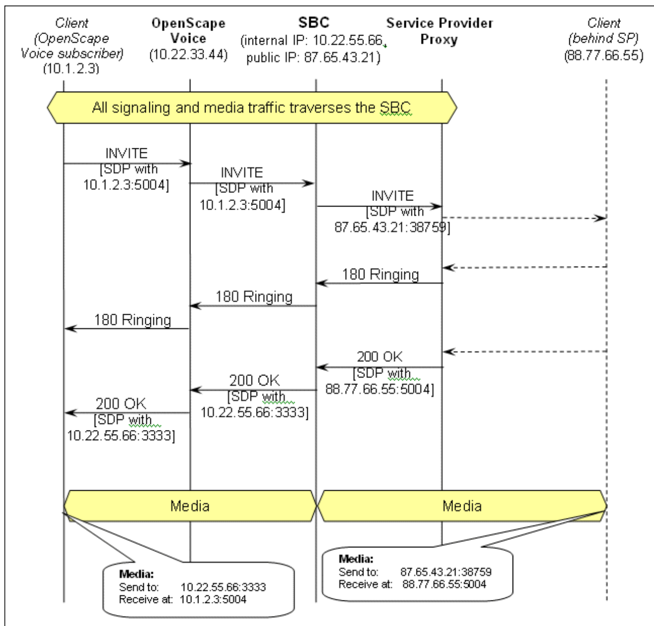
Figure 9 Example SBC at the OpenScope Voice V11 System Boundary
