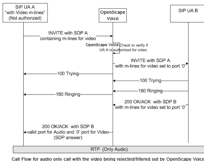
Figure 21: Overview of OpenScape Voice Filtering out Video from the Call
