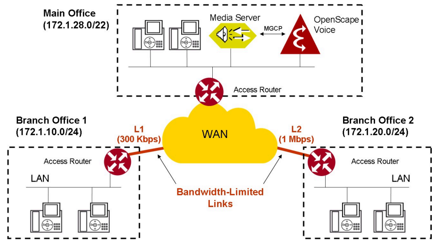
Figure 22: Sample Network Topology Requiring Voice Codec Restriction
