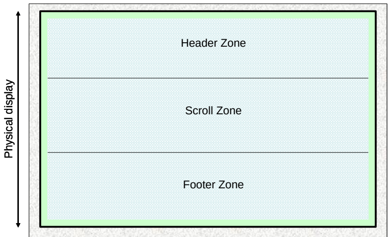
Figure 42: FormattedTextScreen layout
