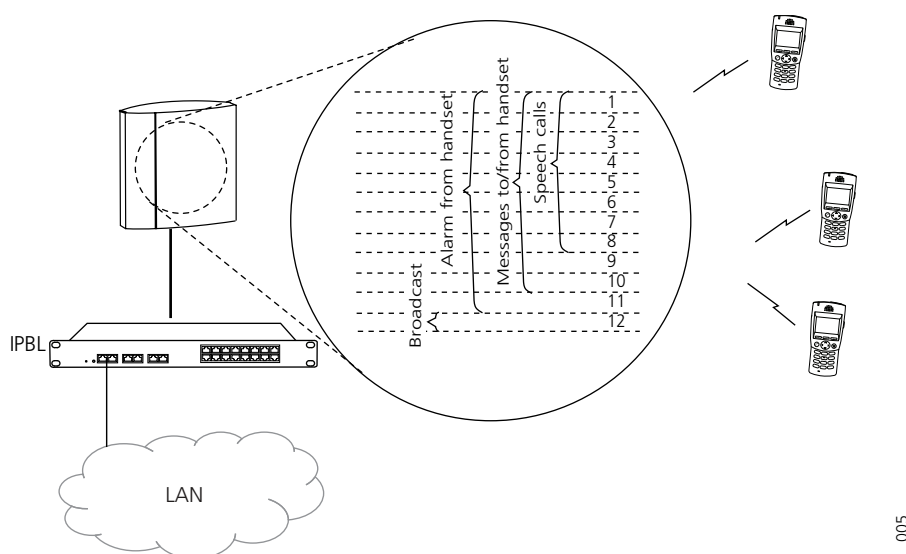
Figure 23. Channel distribution in the DB1/BS3x0 connected to the IPBL
