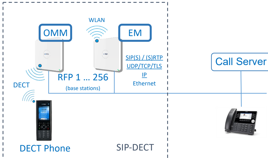
Figure 1: SIP-DECT Architecture Overview - OMM and EM running on RFP
