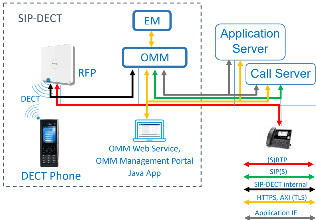
Figure 3: SIP-DECT Protocols
