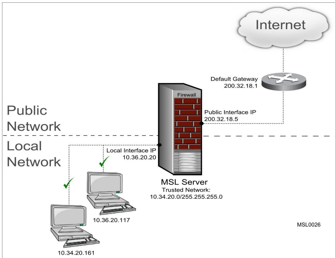
Figure 18: Routing Configuration with Trusted Network
